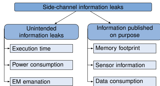
Fig. 4. Types of side-channel information leaks.
